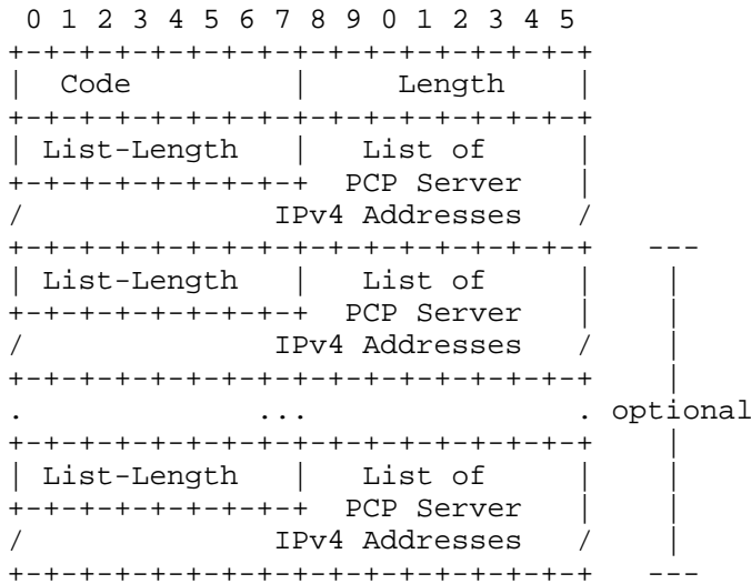
Figure 2: DHCPv4 PCP Server Option
